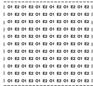
Figure 10. Combined Frame Output from Graphics Controller
